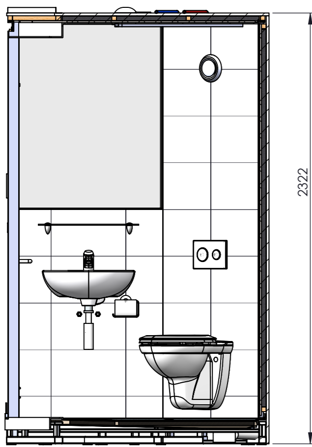
SECTION L-L
