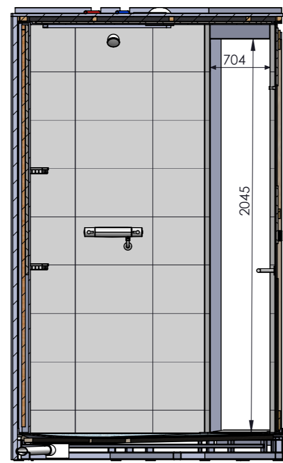
SECTION O-O
